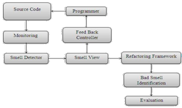
Fig. 2. Architecture Diagram.
