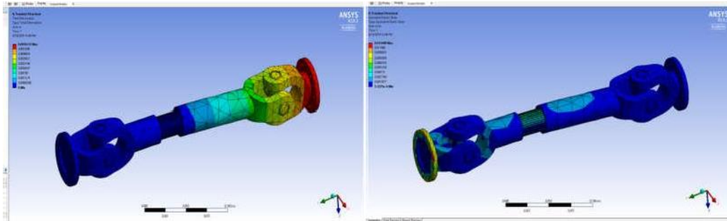
Fig.4.7 Total Deformation
