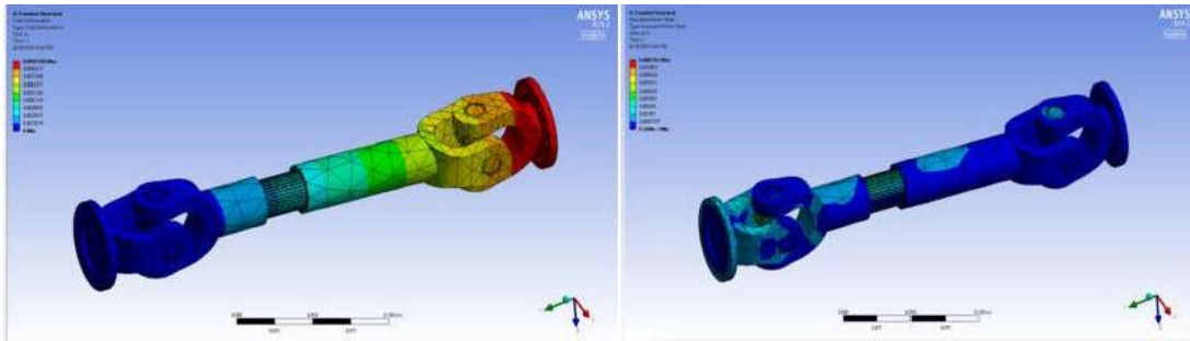
Fig.4.1 Total Deformation
