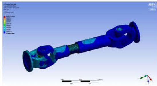
Fig.4.2 Equivalent Strain
