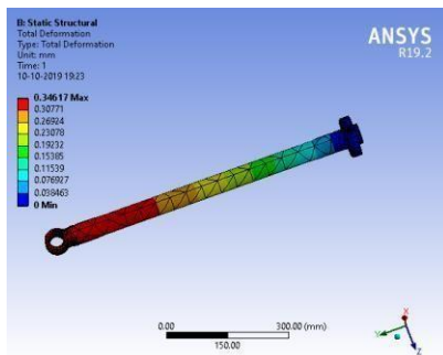
Fig.4.1 Total Deformation
