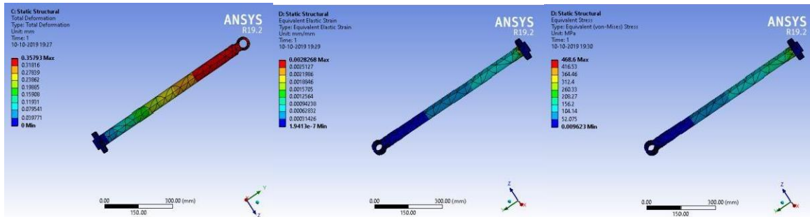
Fig.4.7 Total Deformation
