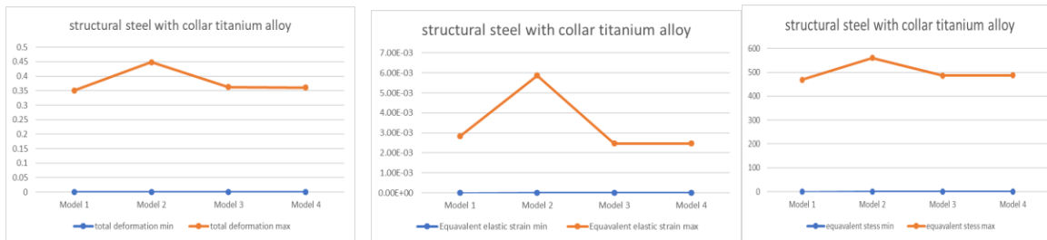
Fig.5.3.1 Total Deformation Fig.5.3.2 Equivalent Elastic Strain Fig.5.3.3 Equivalent Stress
